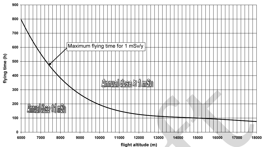
Figure 1: Delimitation of the zone where the annual dose may be higher than 1 mSv as a function of flying time and flight altitude
