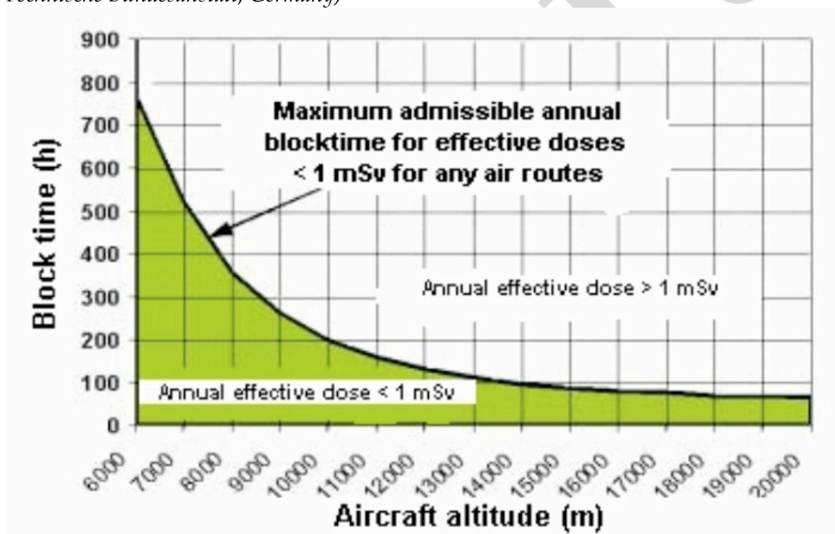
Figure 1: Limiting curve for the keeping of 1 mSv in dependence of the maximum permissible flight hours (block time) and the cruising altitude of the aircraft (Source: Physikalisch-Technische Bundesanstalt, Germany)
